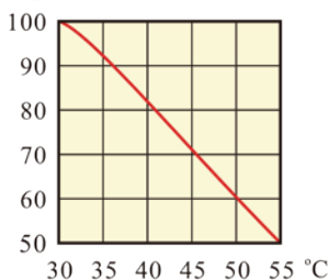
Rated Capacity %
